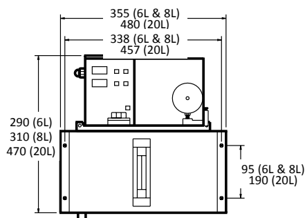
(Note: All dimensions are mm.) 6, 8 and 20 Liter Reservoirs
