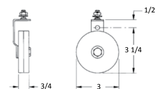
ROTARY BRACKET ASSEMBLY WITH MOUNTING STUD
