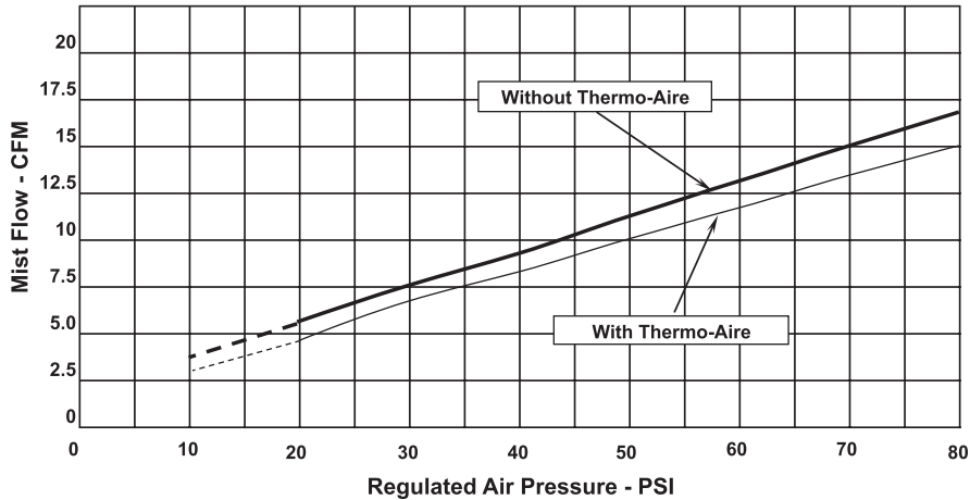
9.7 CFM Nozzle - 3700 Series
